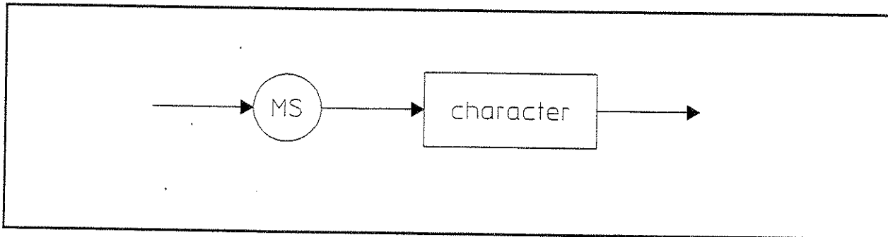
Figure 2-33. MS Syntax Diagram
